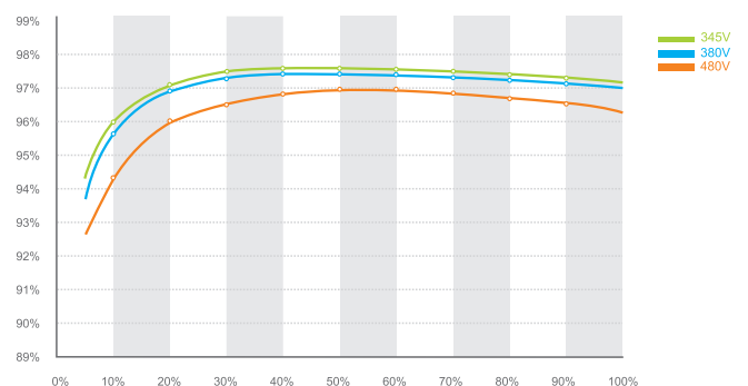
Growatt 11000tl-us efficiency
